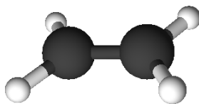
ethylene
